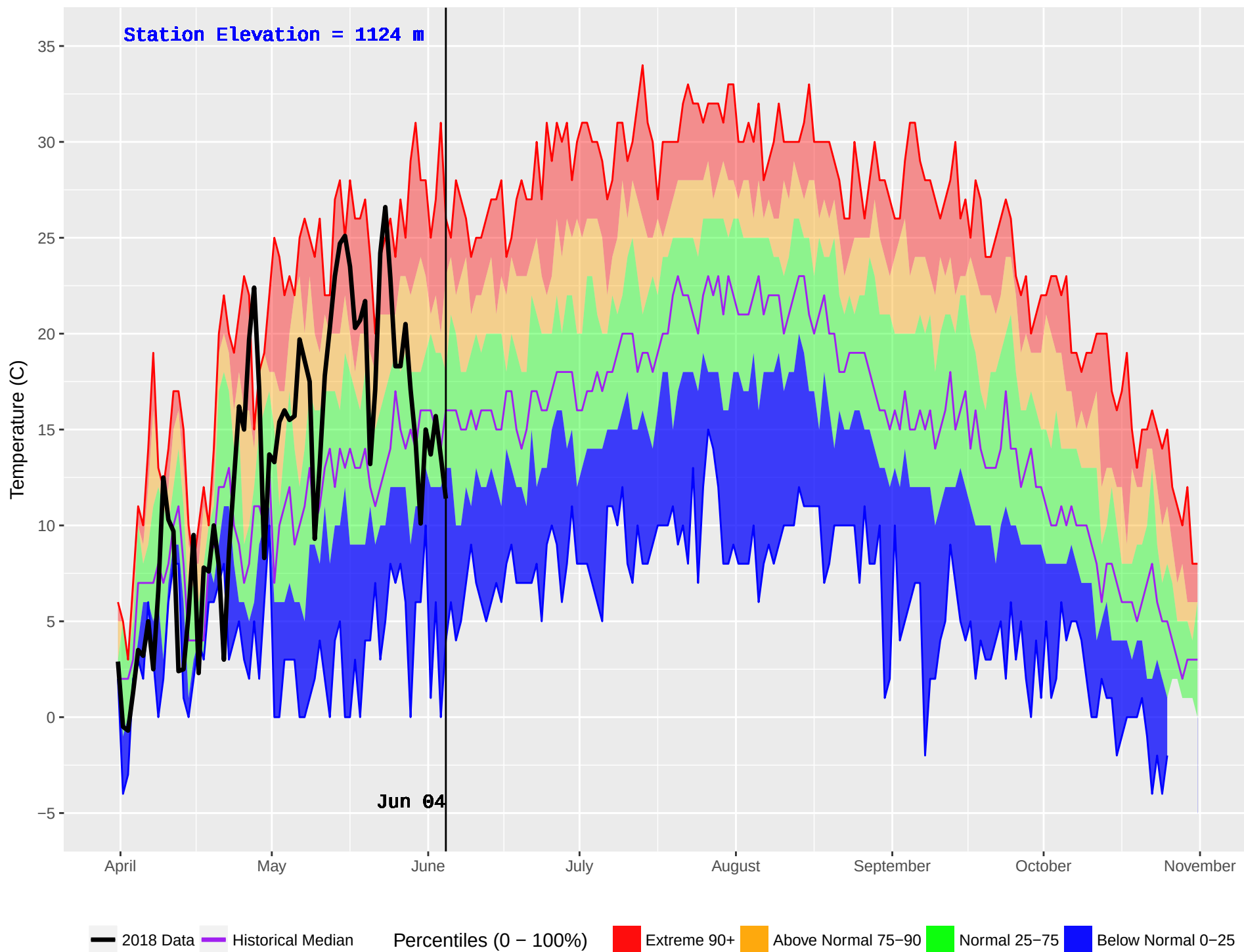
COLDSCAUR LAKE (232) : Historical (1979–2016) and Current (2018) Noon Temperature
